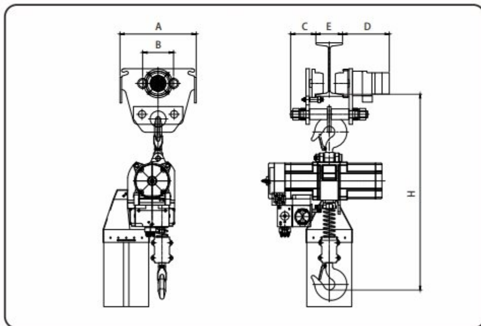
Hoist with trolley
